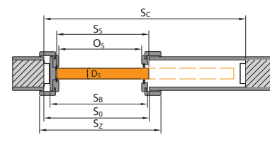
■ FRAMELESS SLIDING SYSTEM
