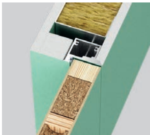
Non-rebated door leaf (outwards outwards) - right door
