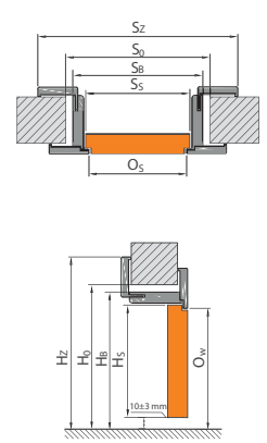
■ DOOR FRAME WITH REVERSED REBATE
